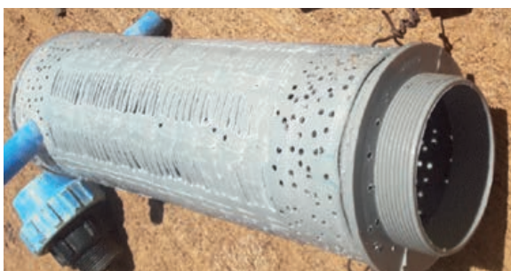
Figure 13: Perforated PVC pipe to protect strainer
