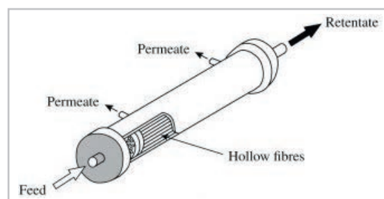
Figure 6: Hollow fibre membrane module (adapted from Doran, 2013)
