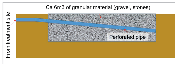
Figure 29: Infiltration trench
